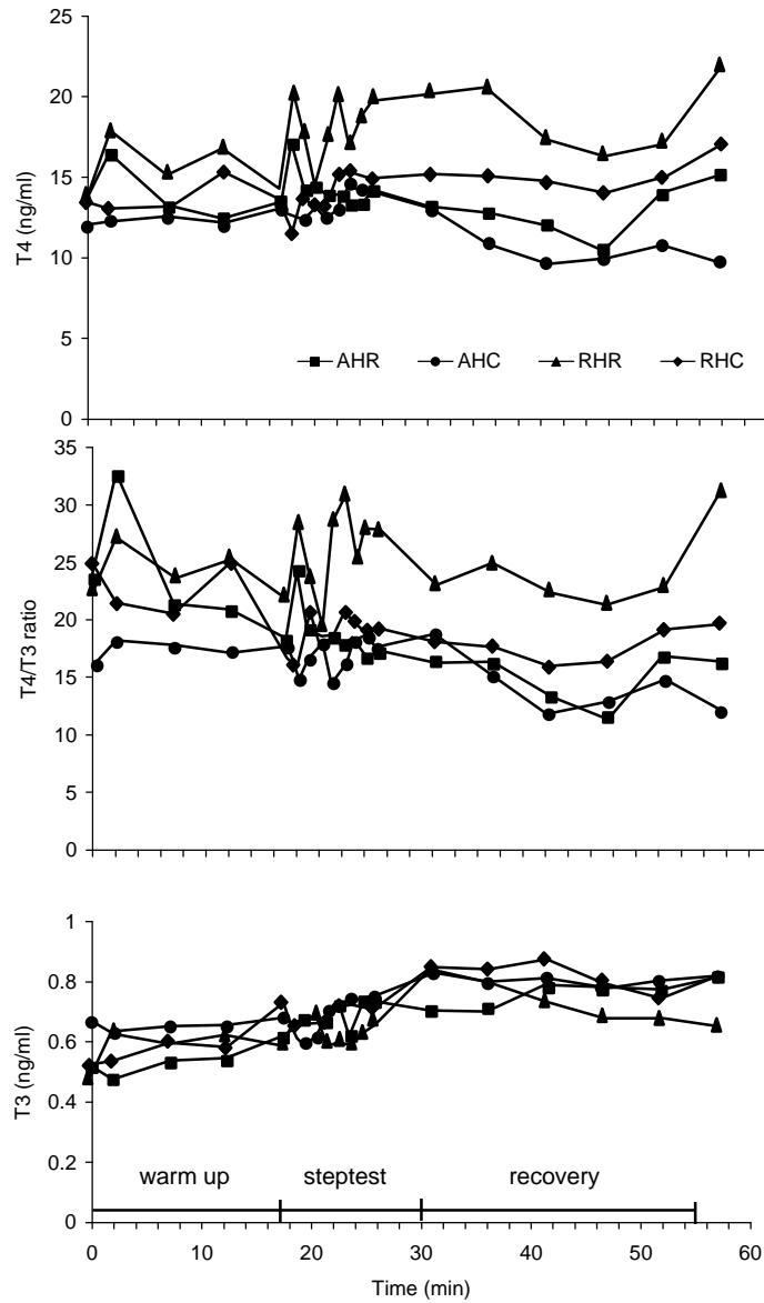
Figure 2. Mean serum concentrations of thyroxine ( T_4 ), triiodothyronine ( T_3 ), and T_4/T_3 ratio in horses fed adequate high roughage (AHR), adequate high concentrate (AHC), 70% of AHR (RHR) or 70% of AHC (RHC) diets during an exercise test.
